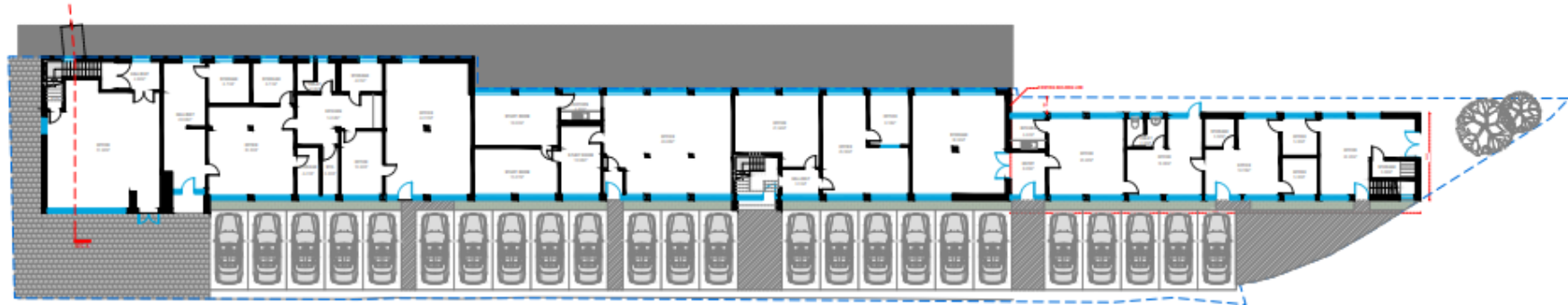
GROUND FLOOR PLAN (BLDG A) S.A. = 188,108'
