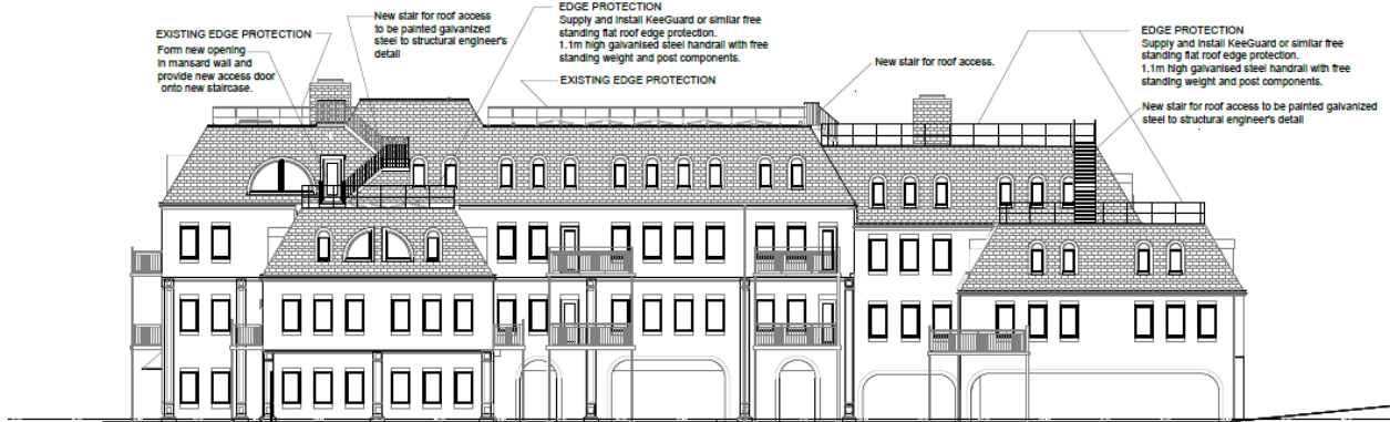
South Elevation - Sunbury Station (Car Park / Station Approach)
